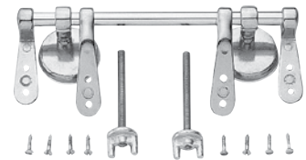
747 € 11,20 Coppia cerniere per sedile WC, in ottone cromato, tipo con tubetto per sedili in legno, con 8 viti in ottone. Couple hinges for WC seat, in C.P. brass, kind with pipe for wooden seats, with 8 brass screws.
