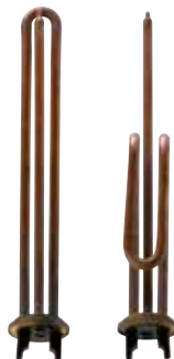
1121 1"1/4 €10,90 Resistenza per scaldabagno attacco con flangia, Watts 1200. Straight heating element for water heater, 1"1/4, flanged cap, Watts 1200.
