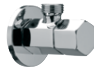
128E 12 38 1/2x3/8 € 17,60 Rubinetto sottolavabo "Esagonale", con vitone ceramico, 1/2x3/8. C.P. brass "Hexagonal" angle valve, with ceramic head valve, 1/2x3/8.
