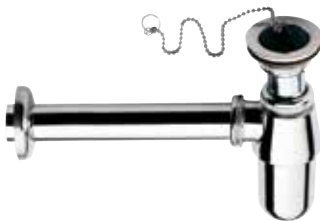
973 Z 1"1/4 € 23,40 Sifone a bottiglia in zama con piletta, per lavabo, 1" 1/4. Bottle trap in zamac with waste, for wash-basin, 1" 1/4.
