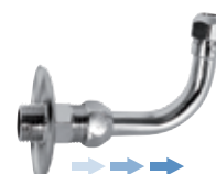
124R 12 10 1/2x10 € 7,10 Curvetta sottolavabo stampata, 1/2x10, allungabile, con rosetta in ottone cromato. C.P. brass forged elbow connection for wash basin, extendible, with flange, 1/2x10.
